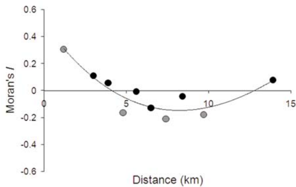
Fig. 2. Spatial autocorrelogram (Moran's I) for density of Feral Pigeons in Poznań. Grey circles indicate spatial autocorrelations significant at \alpha < 0.05 .
