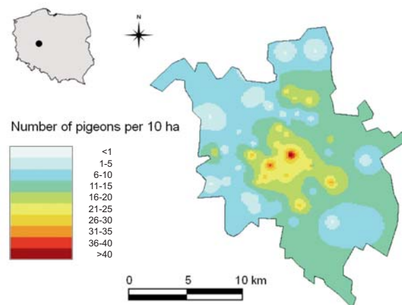
Fig. 1. The interpolated density of the Feral Pigeon in administrative boundaries of Poznań. The interpolation was performed with an inverse distance method in Quantum GIS software.
